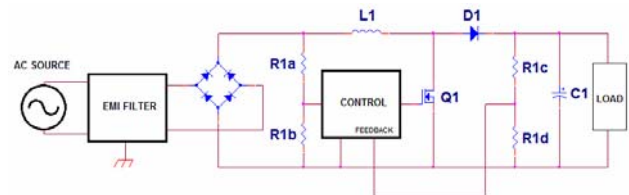
Fig. 2 - Non-isolated PFC stage
