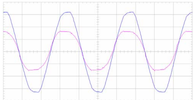
Fig. 1D - Typical input voltage and current waveforms for a PFC circuit.
