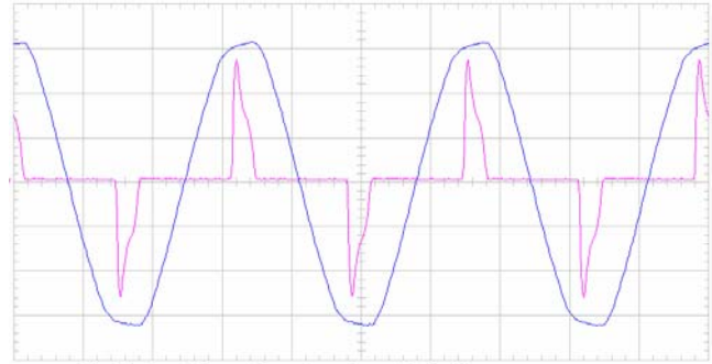
Fig. 1C - Input voltage and current waveforms typical of the bridge rectifier and bulk capacitor combination.
