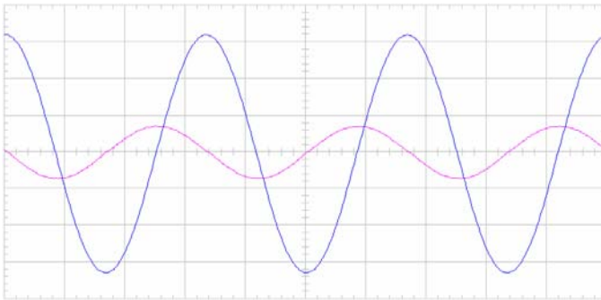
Fig. 1B - Non-Unity Power Factor. A 90 degree phase shift between input current and input voltage is the result of a capacitive load.
